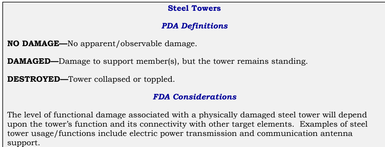
Figure 25. PDA and FDA Definitions and Considerations for Steel Towers
