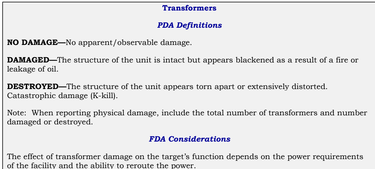
Figure 26. PDA and FDA Definitions and Considerations for Transformers
